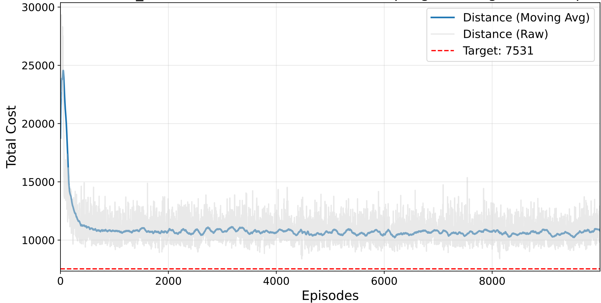
Final NO_MASK Masked AutoRL-SOP (Resampling) Training - ft53.1.sop
